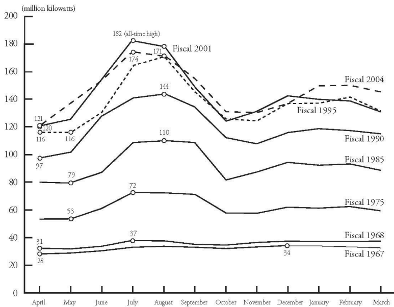
Figure 1. Year-Round Trends in Electricity Use
