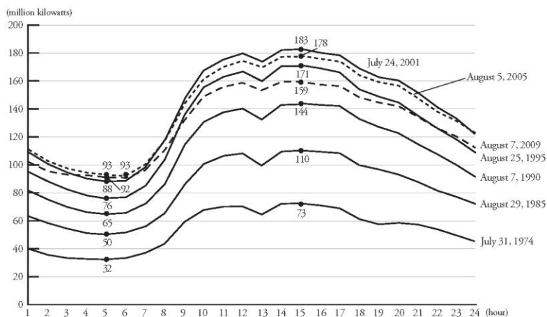
Figure 2. Hourly Trends in Electricity Use on Peak Demand Day
